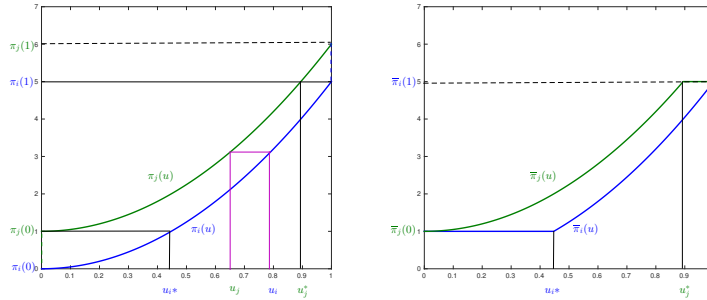
Figure 2.1: Capillary pressure curves (left) and truncated capillary pressures curves (right)
