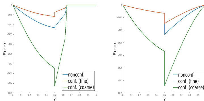
Figure 6.4: Example 1. Error in saturation along a line orthogonal to the interface, nonconforming and conforming (coarse and fine) time-steps. Left T = T_f/20 , right, T = T_f .
