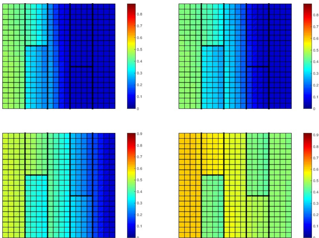
Figure 6.12: Example 3: Saturation u(t) at the bottom face of \Omega , for t = 500 , t = 1000 , t = 2000 and t = 4000
