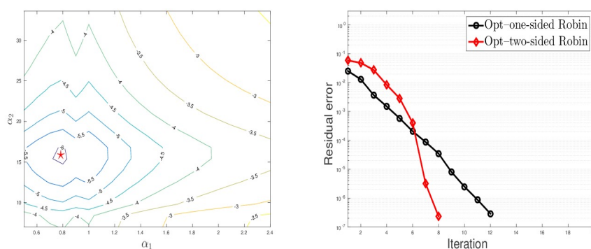
Figure 6.9: Example 2: Left: Level curves for the residual error obtained after 8 iterations for various values of the parameters \alpha_1 and \alpha_2 . The red star shows the optimized parameters. Right: The convergence curves of the optimized Schwarz method with one-sided optimized Robin conditions and two-sided optimized Robin conditions.
