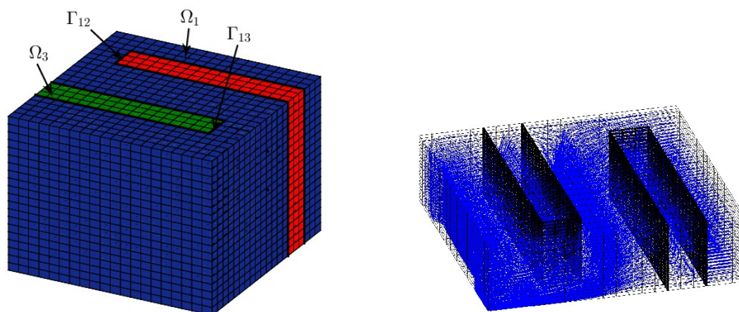
Figure 6.10: Example 3: Left: The geometry and the mesh. Right: Velocity streamlines.
