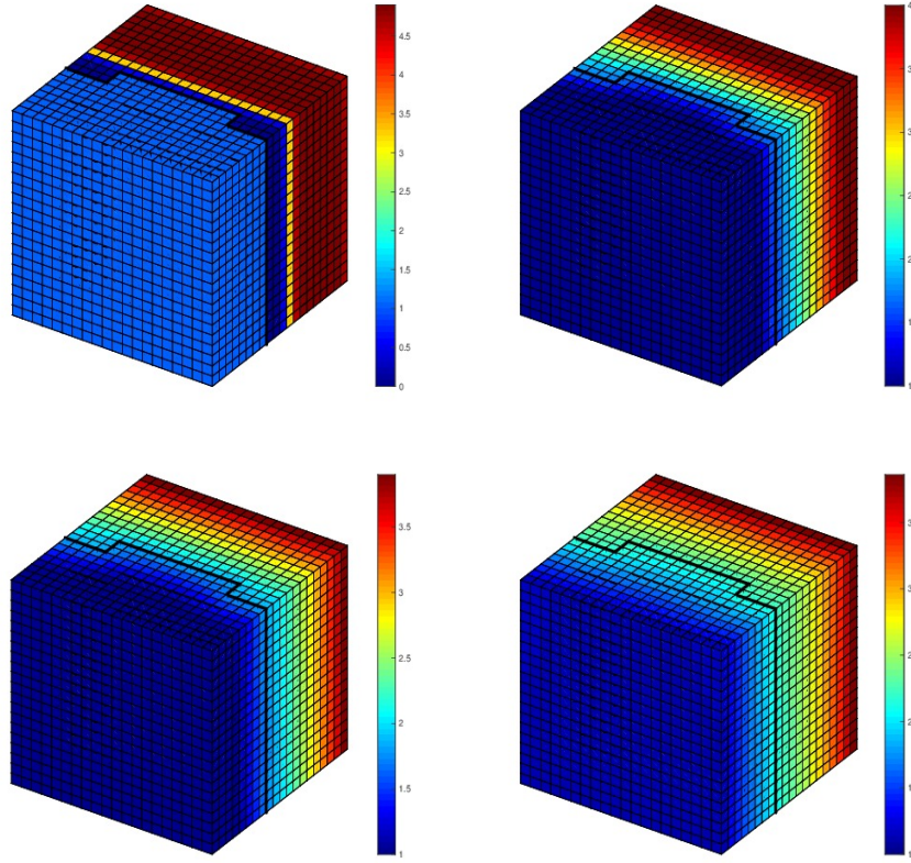
Figure 6.2: Example 1: Capillary pressure \pi(u(t)) , for t = 0.019 , t = 0.3 , t = 0.6 , and t = 3
