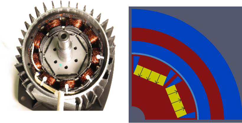
Fig. 1 Real world IPM electric motor (see Acknowledgement) on the left, and a quarter of the cross section of a similar electric motor with 8 magnetic poles that is used in our numerical tests on the right.
