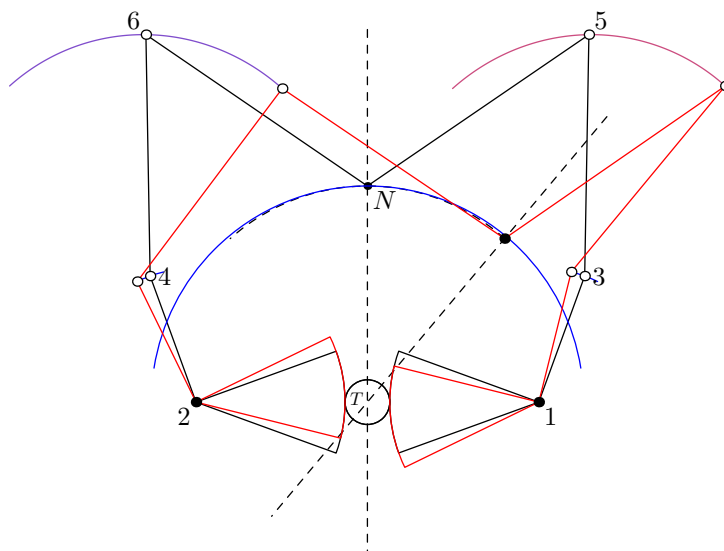
Figure 13: A linkage intermediate between the (supposedly) old and new ones, with a N -path at nearly constant distance from the bell rotation axis.
