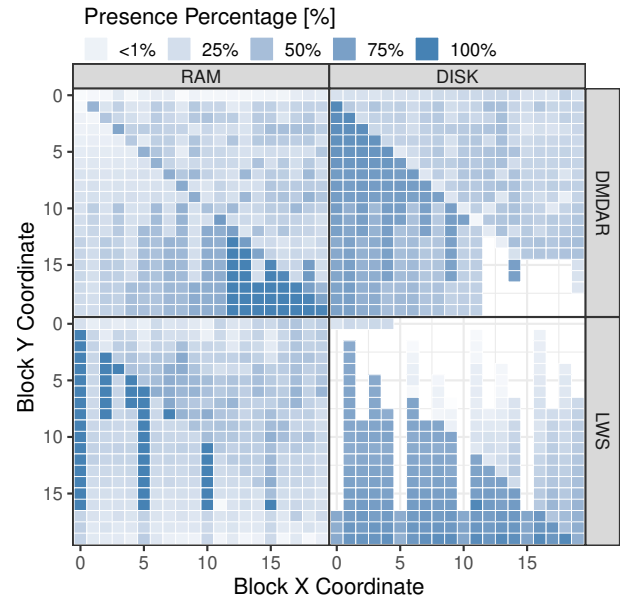
Fig. 14: Heatmaps showing block presence throughout the run.
