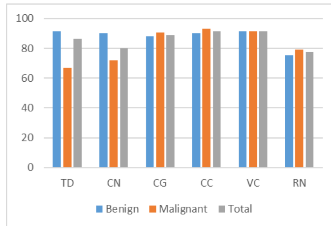
Fig. 4. Accuracy percentage in images classification. Source: Authors
