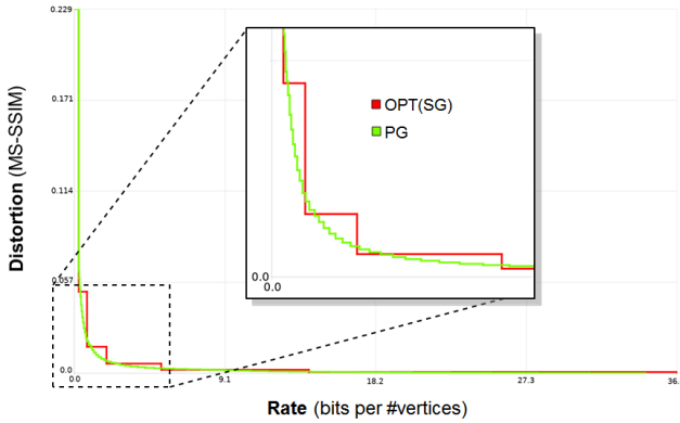
Figure 12: Rate-distortion curves for LOD sequences without texture costs on the re-atlased Tiger. PG (Green, agony: 0.133725) is a better curve than the OPT(SG) (Red, agony: 0.159542).
