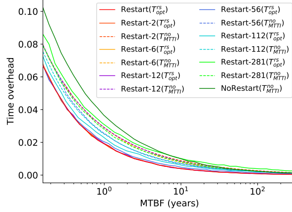
Figure 11: Comparison of restart strategy with restart only every 2, 6, 12, 56, 112, or 281 dead proc., with T_{opt}^{rs} and T_{MTTI}^{no} .
