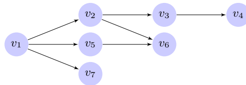
Figure 1: DAG example.
