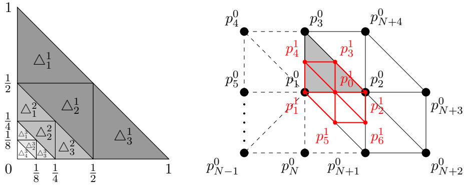
Figure 3: Left: decomposition of the unit triangle \Delta in smaller triangles corresponding to the splines rings of the adaptive Gaussian quadrature \text{AG}(p, L) for L = 3 . Right: illustration of the vertex configuration, with numbering as in Table 1 (black straight and dashed lines) with a vertex p_1^0 of valence N in the neighborhood of the edge e connecting p_1^0 and p_2^0 . The red lines indicate the new vertices and edges in the 1-neighborhood of p_0^1 after one level of subdivision.
