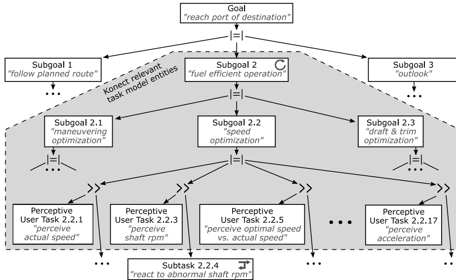
Fig. 2. Part of a task model for officers on ship bridges. Due to space restrictions many parts are omitted, indicated by dots (...). Aspects that are relevant for the Konekt method are within the gray box. Graphical notation based on HAMSTERS notation. |=| indicates order independent execution of subtasks. >> indicates sequential execution of subtasks.
