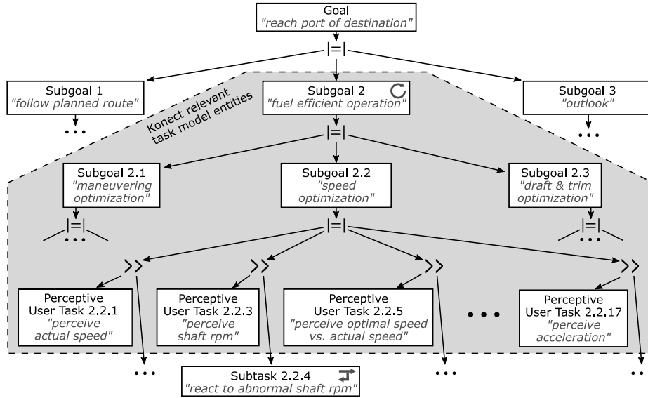
Fig. 2. Part of a task model for officers on ship bridges. Due to space restrictions many parts are omitted, indicated by dots (...). Aspects that are relevant for the Konec method are within the gray box. Graphical notation based on HAMSTERS notation. |=| indicates order independent execution of subtasks. >> indicates sequential execution of subtasks.
