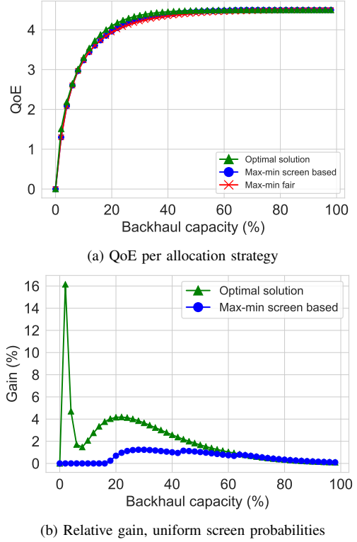
Fig. 4: Comparison of allocation strategies with uniform screen probabilities, QoE from III-C2
