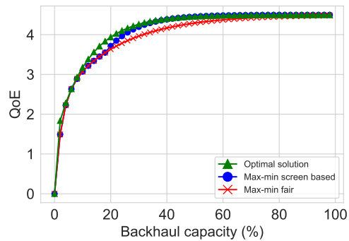
(a) QoE per allocation strategy
