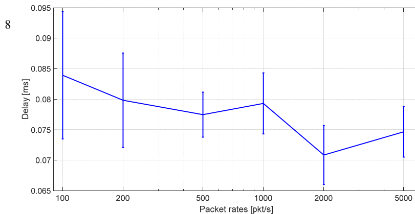
Fig. 3. Obtained delays under different packet rates with disabled emulator.
