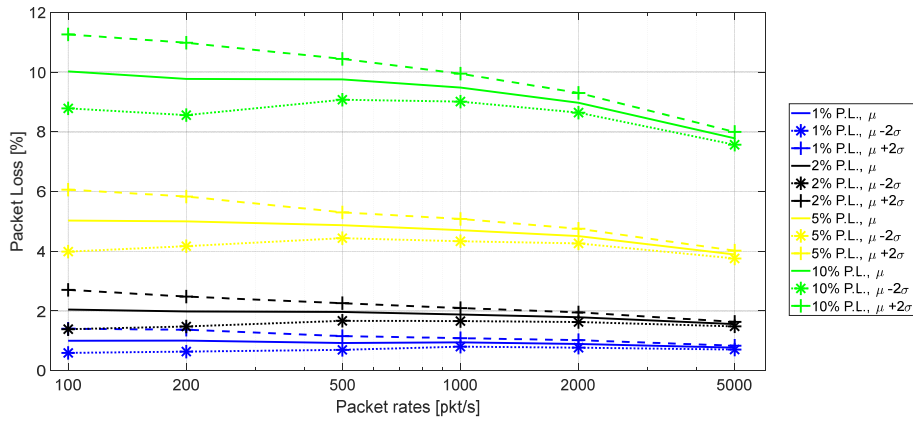
Fig. 6. Obtained packet losses under different packet rates with NetEM emulator.
