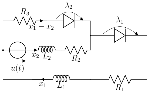
Figure 2.9: A circuit with two ideal diodes and a voltage source
