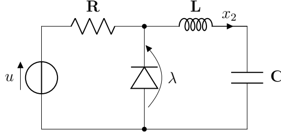
Figure 2.15: RLCD circuit with a voltage source.
