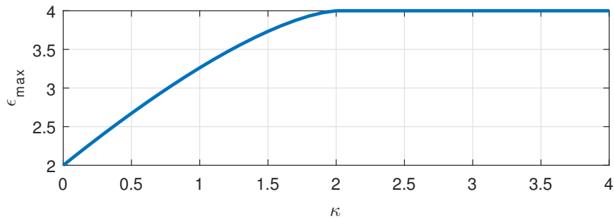
Figure 2.19: Relation between \kappa and optimal value of (\mathbf{Q}_\kappa)
