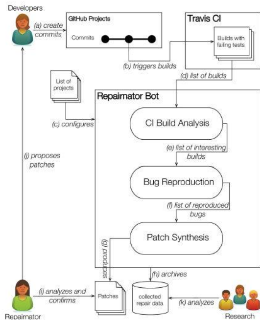
Figure 1. The Repairator workflow.
