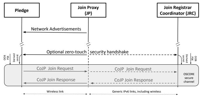
Fig. 5. Exchanges taking place during the join process. Physical links are depicted with solid, logical connections with dashed lines. OOB stands for out-of-band.
