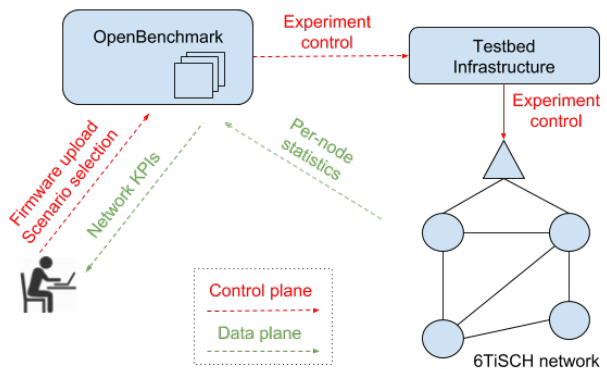
Fig. 1. Overview of OpenBenchmark functionality.
