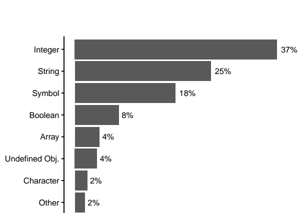
Figure 1. Distribution of literals over data types
