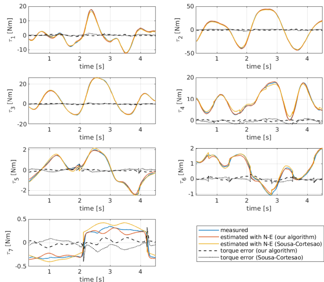
Fig. 1. Comparison between measured joint torques during a validation trajectory (blue solid lines) and estimated torques generated from a N-E routine using the \hat{\mathbf{p}} parameters from our parameter retrieval method in [1] (solid red lines) and the parameters \boldsymbol{\delta} from the LMI-SDP framework in [3] (solid yellow lines). The torque errors are reported as well.
