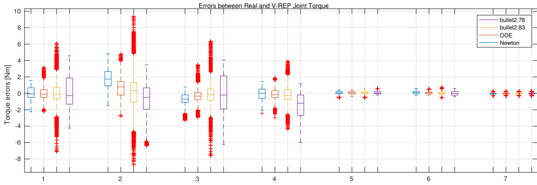
Fig. 6. Torque errors (w.r.t. the real robot) of the physics engines Bullet 2.78, Bullet 2.83, ODE, and Newton in V-REP during an experiment with the Panda robot for each of its 7 joints. The boxes indicate mean values of the errors while the bars denote their standard deviations.
