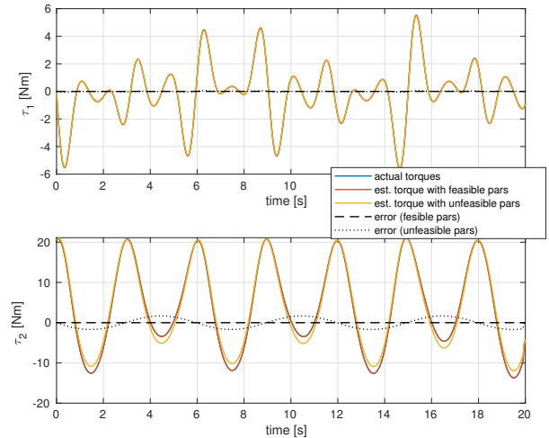
Fig. 9. Validation of estimated parameters in Table VII. A N-E routine fed with the feasible parameters \hat{p} and with some unfeasible parameters \hat{p}' returns similar estimated torques (respectively, red and yellow lines) along the motion. When comparing these estimates with the actual torques recorded along a sinusoidal joint trajectory (blue lines, almost overlapped by the red line), we notice that both sets provide a good torque estimation.
