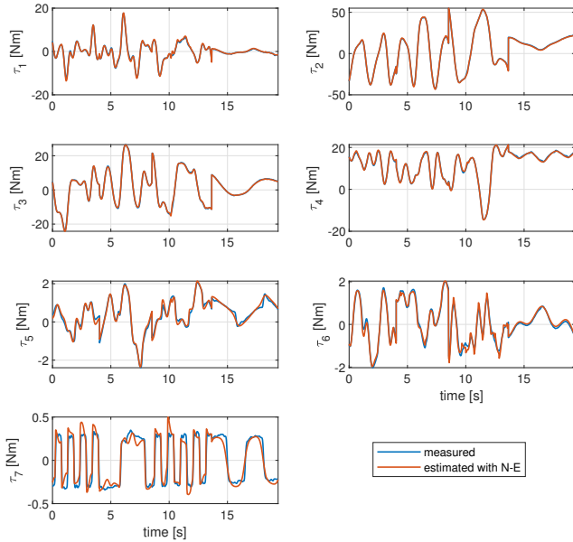
Fig. 5. Comparison between the torques \hat{\tau}_{ne} (including friction \hat{\tau}_f ) from the N-E dynamic model and the ones retrieved from the the joint torque sensors. The overlapping of two signals shows the quality of the obtained parameters estimation \hat{p} .
