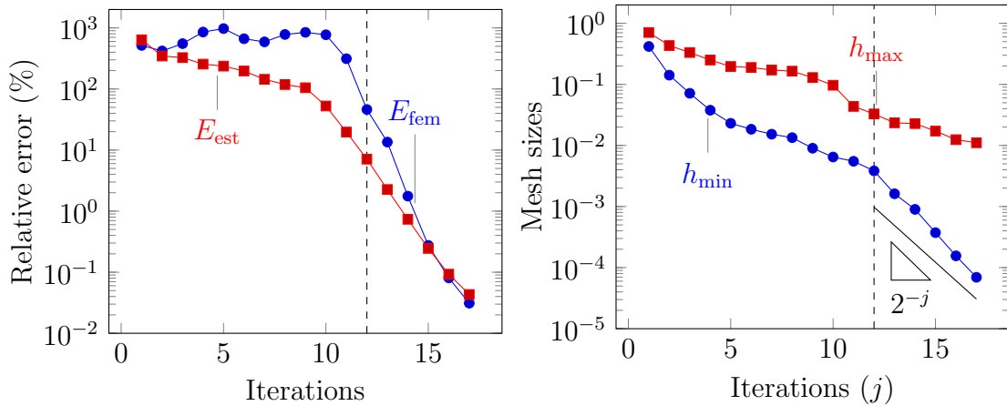
FIGURE 14. Behaviors of the estimated and approximate analytical errors and mesh sizes in the adaptive procedure for the scattering problem of Section 6.2, \mathcal{P}_4 elements and k = 120\pi
