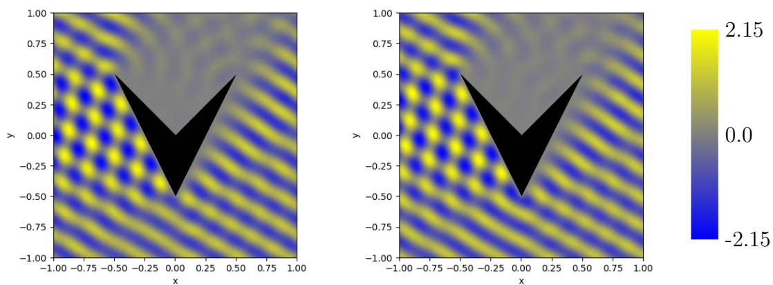
FIGURE 10. Scattering problem with \nu = \pi/3 : real (left) and imaginary (right) parts of the solution for k = 10\pi
