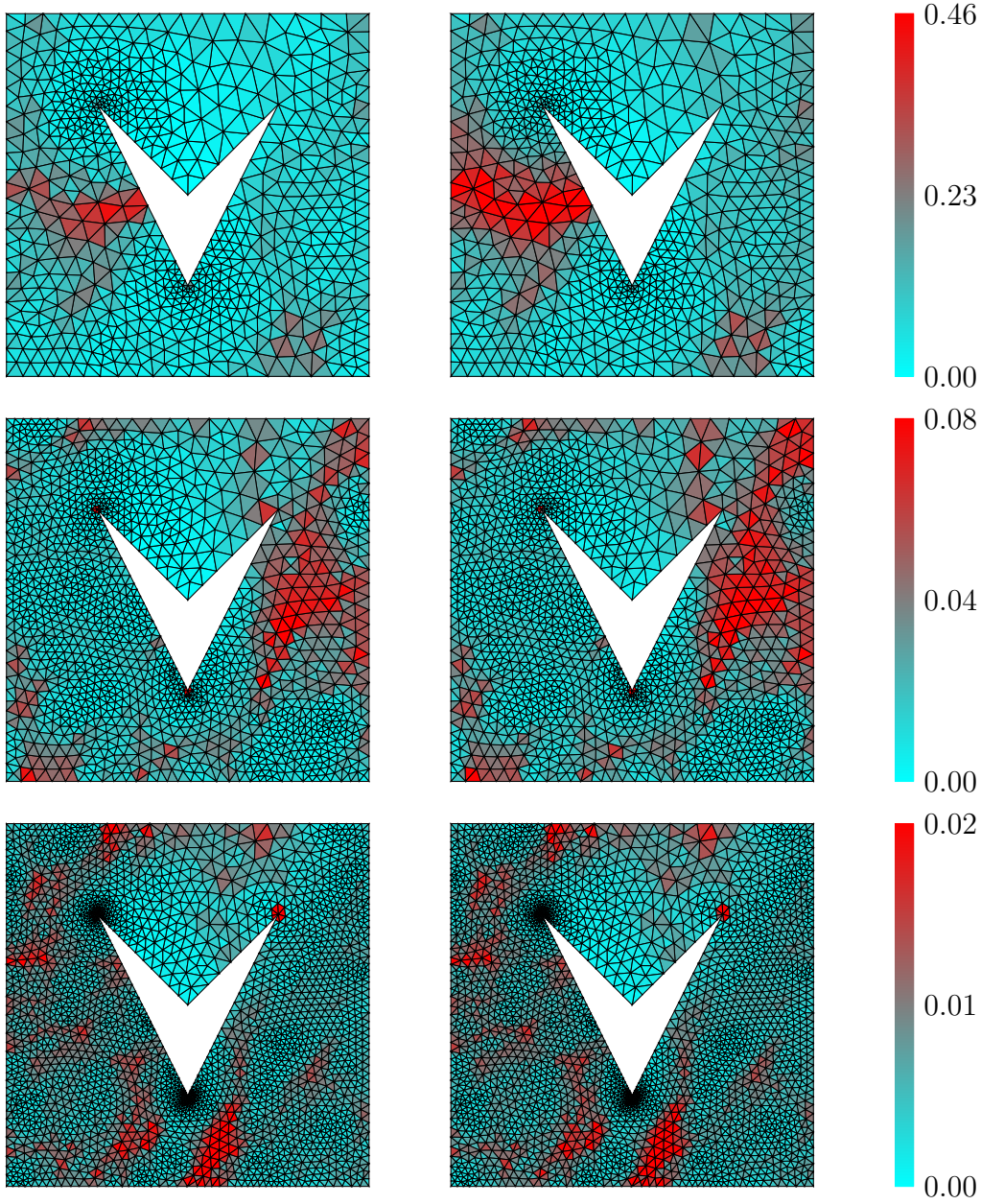
FIGURE 9. Estimators \eta_K (left) and elementwise errors \|\tilde{u}_h - u_h\|_{1,k,K} (right) for the scattering problem of Section 6.2 for k = 10\pi with \mathcal{P}_3 elements
