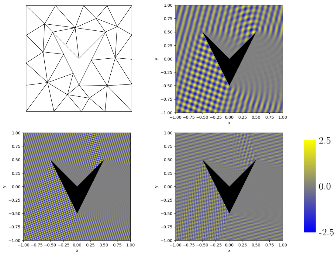
FIGURE 11. Initial mesh for the adaptivity experiment and real part of reference solution for different wavenumbers. Top right panel: k = 20\pi . Bottom left panel k = 60\pi . Bottom right panel k = 120\pi
