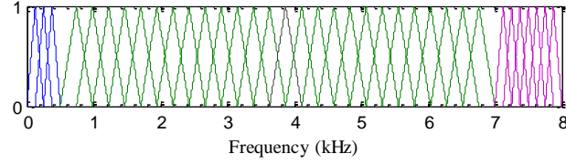
Fig. 5. 16 sub-band linear filter design
