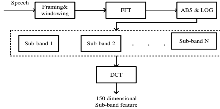
Fig. 1. Sub-band feature extraction
