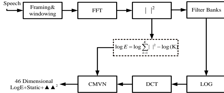
Fig. 3. Feature extraction
