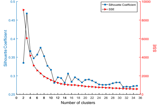
Fig. 1. SSE and Silhouette Coefficient value in different K of ORDS.
