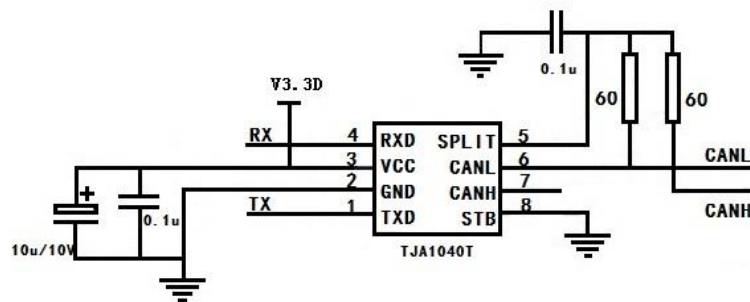
Fig. 2. CAN/TTL Converter circuit
