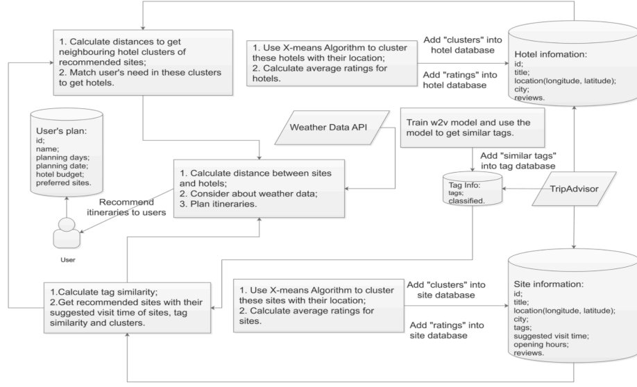
Fig. 1. The workflow for a recommender
