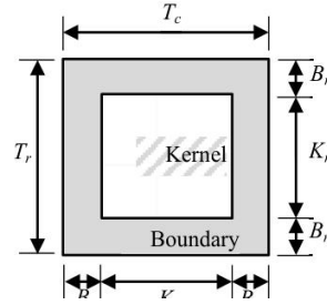
Fig. 2. A block containing the kernel area and the boundary area
