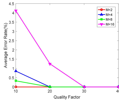
Fig.5. anti-compression performance
