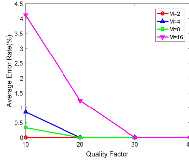
Fig.5. anti-compression performance
