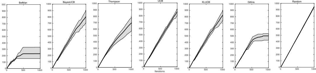
Fig. 2. Evolution of number of suboptimal draws for 20-arm Bernoulli bandit with expected rewards [0.25 0.22 0.2 0.17 0.17 0.2 0.13 0.13 0.1 0.07 0.07 0.05 0.05 0.05 0.02 0.02 0.01 0.01 0.01] for 1000 iterations.
