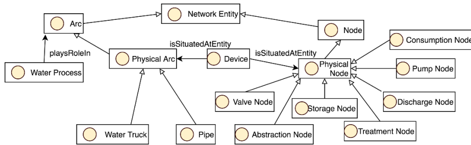
Figure 3 Water Catchment Model
