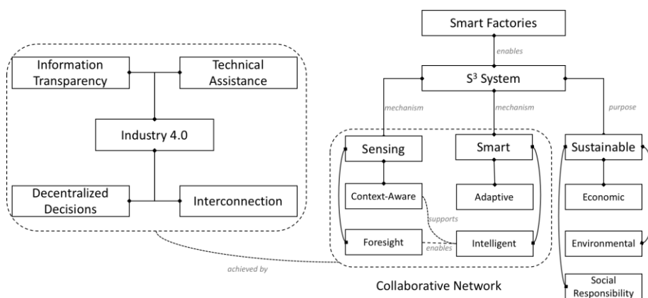
Figure 1. Collaborative Network conceptual model.
