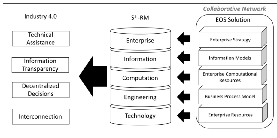
Figure 3 Reference Framework, EOS Solution as Industry 4.0 catalyst
