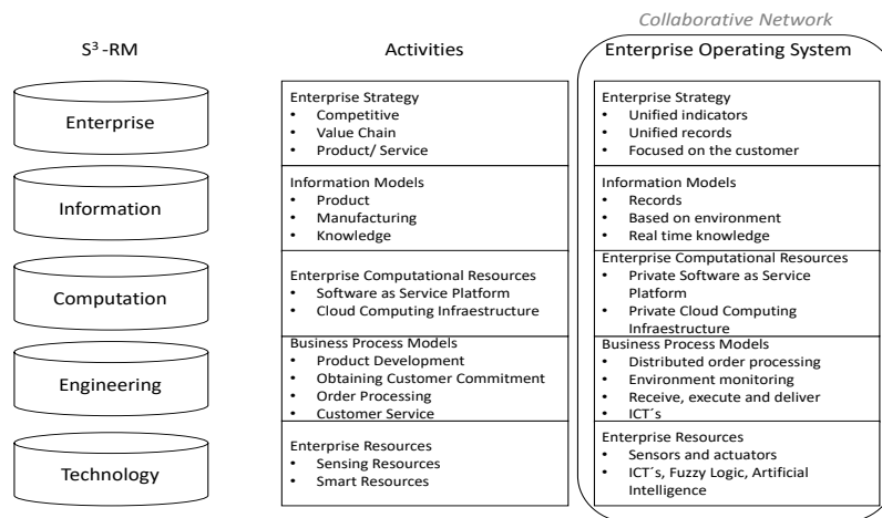
Figure 2 Enterprise Operating System solution
