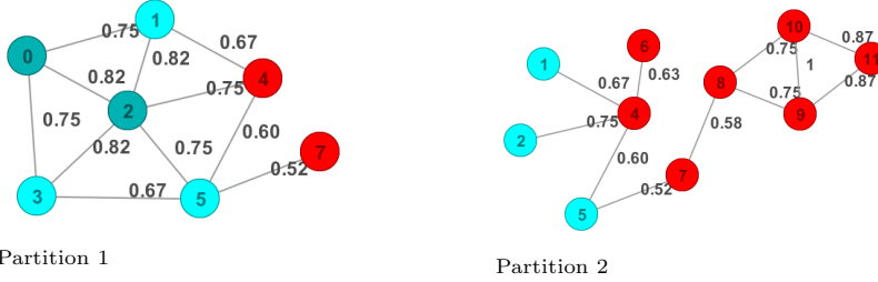
Fig. 4: The partitioned graph G used in the running example in Section 3
