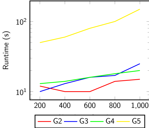
Fig. 9: Impact of the batch size on the running time of DISCAN ( \epsilon=0.5 , \mu=3 )
