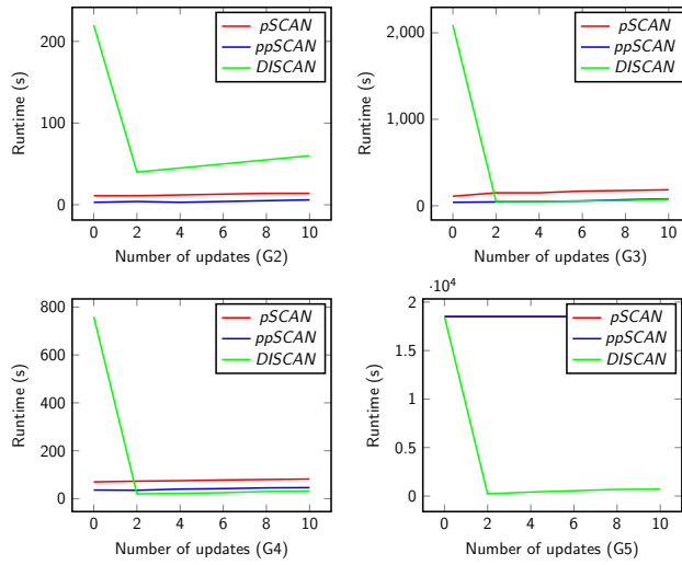
Fig. 7: Impact of the number of updates on the processing time of the pSCAN, ppSCAN and DISCAN ( \epsilon=0.5 , \mu=3 )
