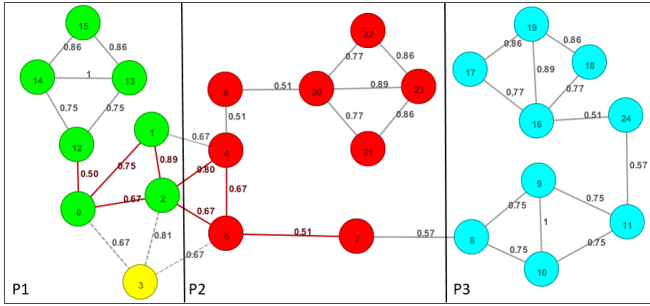
Fig. 5: A partitioned graph G (P1, P2, P3), affected vertices, edges when deleting vertex 3
