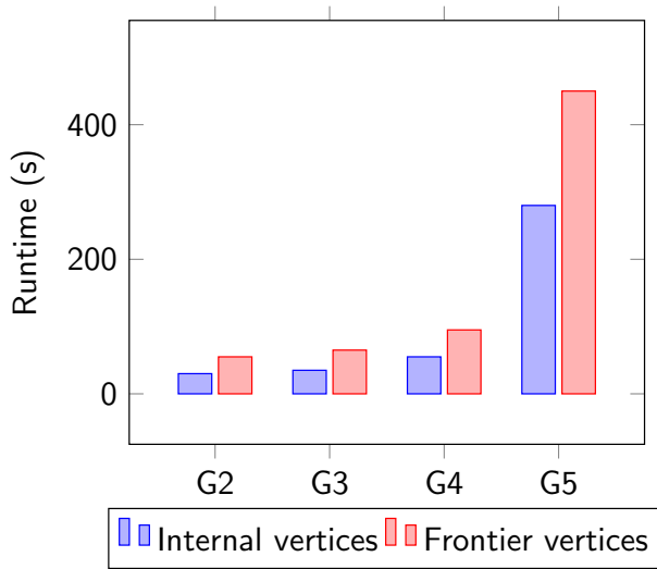
Fig. 10: Impact of the vertices' type (internal or external) on the processing time ( \epsilon=0.5 , \mu=3 )
