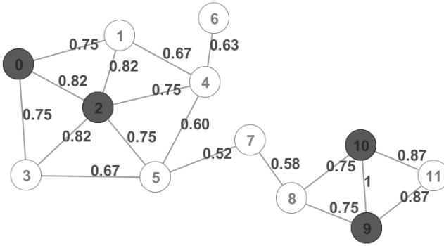
Fig. 1: Running example ( \epsilon = 0.7 and \mu = 3 ).
