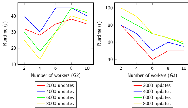
Fig. 8: Impact of the workers' number on the processing time of DISCAN ( \epsilon=0.5 , \mu=3 )
