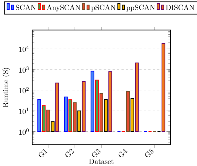
Fig. 6: Impact of the graph size on the processing time of SCAN variants and DISCAN
