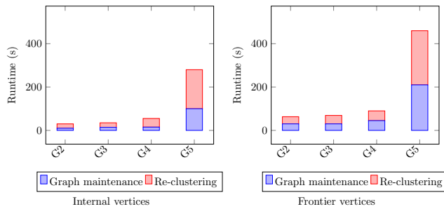
Fig. 11: Performance of DISCAN steps ( \epsilon=0.5 , \mu=3 )
