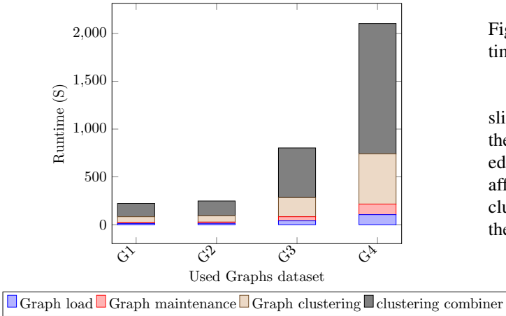
Fig. 7: Performance of DSCAN phases
