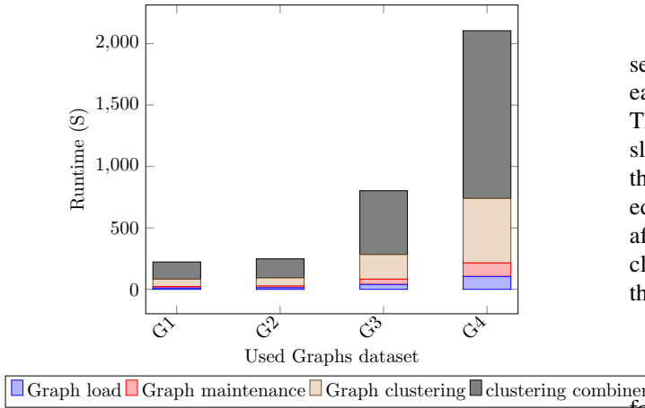
Fig. 7: Performance of DSCAN phases
