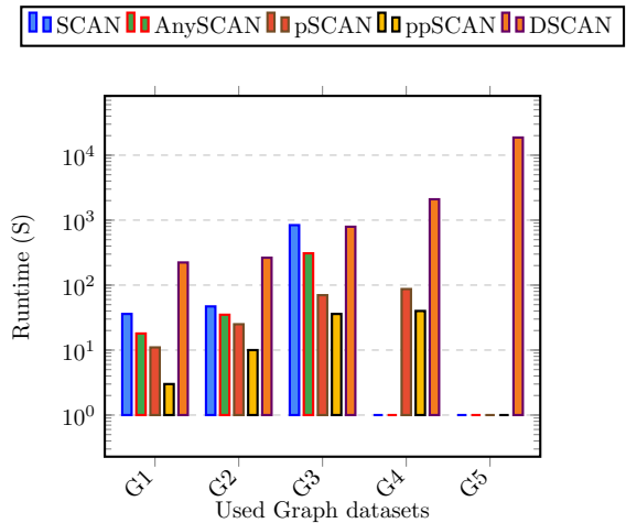
Fig. 4: Impact of the graph size on the processing time of both SCAN and DSCAN
