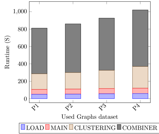
Fig. 8: Impact of the partitioning step on DSCAN response time ( \epsilon=0.5 , \mu=3 )
