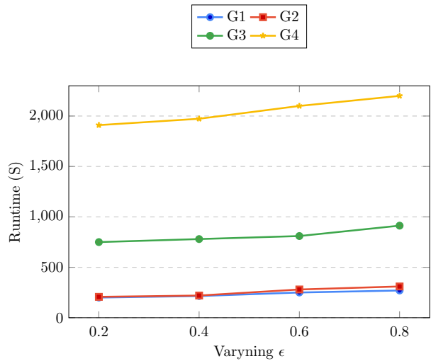
Fig. 6: Impact of the value of \epsilon size on the running time of DSCAN
