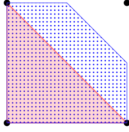
Figure 3: Sets \text{conv}(\mathcal{Y}(\mathbf{x})) and \bar{\mathcal{Y}}(\mathbf{x}) illustrated on an example. Here, \mathcal{Y}(x) = \{y \in \{0, 1\}^2 \mid y_1 + y_2 \leq 1.5 - x\} , \bar{\mathcal{Y}}(x) = \{y \in [0, 1]^2 \mid y_1 + y_2 \leq 1.5 - x\} and x = 0 .
