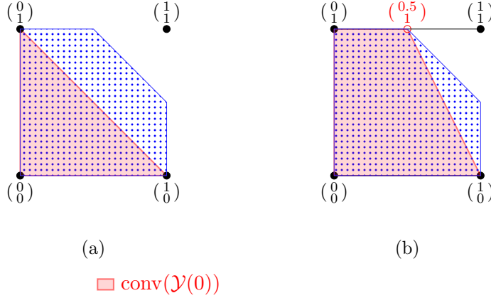
Figure 4: Illustration of Example 2.1 and the implications of Assumption 2.1. In case (a), \mathcal{Y} = \{0, 1\}^2 and \text{conv}(\mathcal{Y}(0)) = \text{conv}\left\{\begin{pmatrix} 0 \\ 0 \end{pmatrix}, \begin{pmatrix} 0 \\ 1 \end{pmatrix}, \begin{pmatrix} 1 \\ 0 \end{pmatrix}\right\} , whose extreme points are a subset of the extreme points of \text{conv}(\mathcal{Y}) . In case (b), \mathcal{Y} = [0, 1] \times \{0, 1\} and \text{conv}(\mathcal{Y}(0)) = \text{conv}\left\{\begin{pmatrix} 0 \\ 0 \end{pmatrix}, \begin{pmatrix} 0 \\ 1 \end{pmatrix}, \begin{pmatrix} 1 \\ 0 \end{pmatrix}, \begin{pmatrix} 0.5 \\ 1 \end{pmatrix}\right\} . The point \begin{pmatrix} 0.5 \\ 1 \end{pmatrix} is not an extreme point of \text{conv}(\mathcal{Y}) .
