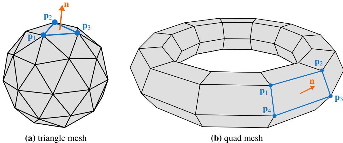
Figure 3.1: Polygonal meshes — Since each face of a polygonal mesh is planar, its normal \mathbf{n} can be computed as (\mathbf{p}_3 - \mathbf{p}_2) \times (\mathbf{p}_2 - \mathbf{p}_1) , where \mathbf{p}_{1:3} are any three vertices of the face.
