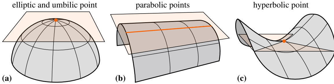
Figure A.4: Surface categorization based on Gaussian curvature.
