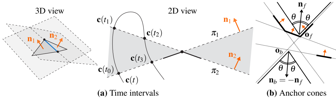
Figure 3.7: Spatial partitioning — (a) A given edge is on the contour generator if the viewpoint trajectory \mathbf{c}(t) is inside the intersection (in grey) of one positive and one negative half-space defined by the face supporting plane \pi_1 and \pi_2 , i.e., during the time intervals [t_0, t_1] and [t_2, t_3] in this example. (b) The front and back-facing anchored cones are defined by their center \mathbf{o}_{f|b} , an opposite normal \mathbf{n}_f = \mathbf{n}_b and a common half opening angle \theta , here visualized in 2D for four oriented segments.
