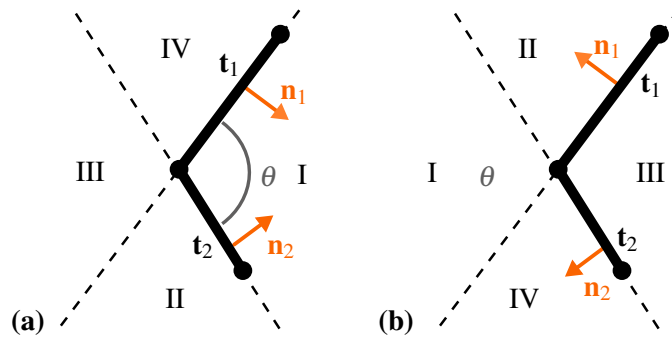
Figure B.1: Concave/convex edge — Cross-section plane for a mesh edge between triangles t_1 and t_2 , with normals \mathbf{n}_1 and \mathbf{n}_2 . The cross-section is some 3D plane perpendicular to the edge between the two triangles. The two faces divide space in four quadrants: I,II,III, and IV. For example, I is the set of points in front of both faces, and II is in front of t_1 and behind t_2 . (a) Concave case: \theta < \pi . Each face is in front of the other. In this case, the edge cannot be a visible contour. (b) Convex case: \theta > \pi . Each face is behind the other.
