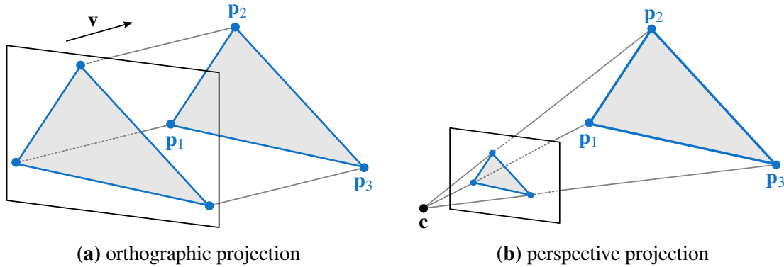
Figure 3.2: Projections — The triangular face formed by the vertices \mathbf{p}_1 , \mathbf{p}_2 and \mathbf{p}_3 is viewed (a) under orthographic projection along the view direction \mathbf{v} , and (b) under perspective projection of center \mathbf{c} .
