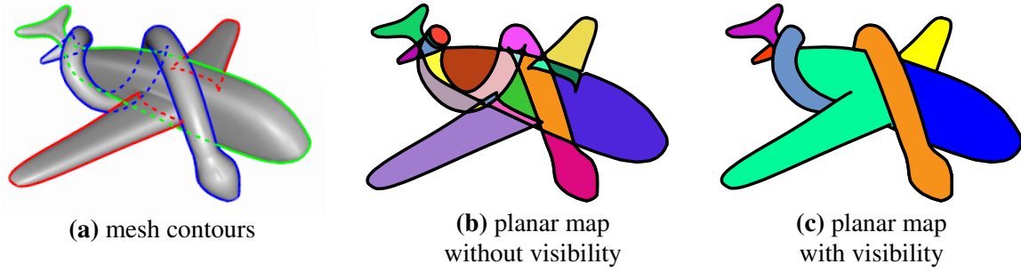
Figure 6.7: Planar Map — Starting from the projected mesh contours (a), the Planar Map corresponds to the partition into cells of the 2D plane induced by these curves (b). If only visible mesh faces are inserted in the Planar Map or snaxels are used, occluded contours will be discarded (c).
