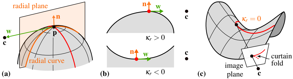
Figure 7.7: Radial curvature — (a) The radial curvature \kappa_r(p) is the curvature of the radial curve at p ; (b) \kappa_r is necessarily positive for visible contours (top) otherwise it would be locally occluded by the surface (bottom), and zero at curtain folds (c).
