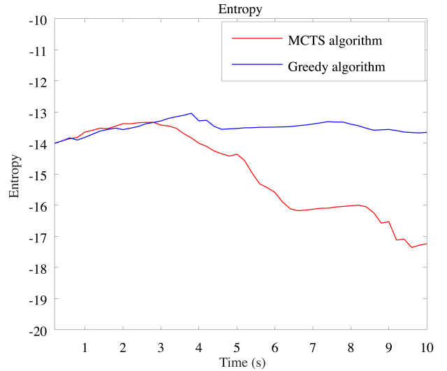
Fig. 14 Entropy over time for the MCTS algorithm and the greedy algorithm with the entropy criterion.
