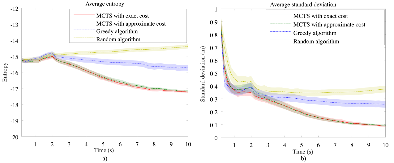
Fig. 17 a) Average entropy and 95% confidence interval over time of the 4 algorithms with the entropy criterion over all 200 experiments. b) Average standard deviation and 95% confidence interval over time with the standard deviation criterion of the 4 algorithms over all 200 experiments.
