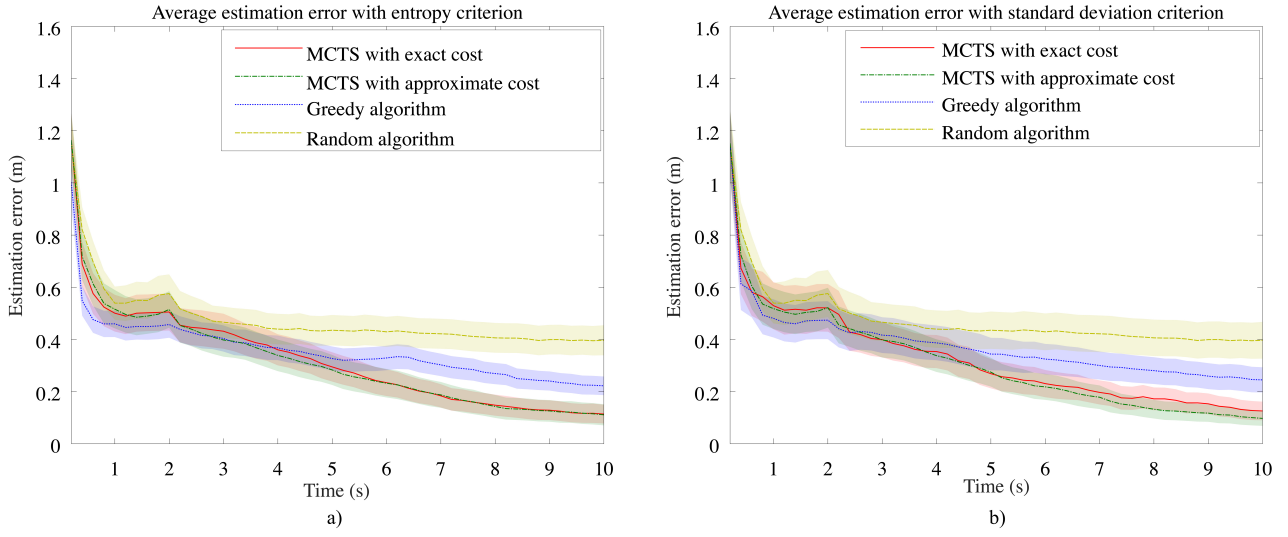
Fig. 18 a) Average estimation error and 95% confidence interval over time of the 4 algorithms with the entropy criterion over all 200 experiments. b) Average estimation error and 95% confidence interval over time of the 4 algorithms with the standard deviation criterion over all 200 experiments.
