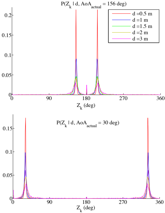
Fig. 2 Distribution of the measured AoA when the actual source is at different angles 156° (top) and 30° (bottom) and different distances from the microphone array.
