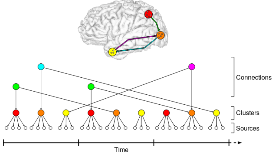
Figure 1: The Bayesian network used to model cortical activity of a simplified brain model. The top panel presents the anatomical model which contains 11 sources illustrated by the small white circles at each time instant, 3 source clusters illustrated by the red, orange, and yellow larger circles, and 3 connections illustrated by the green, teal, and pink arrows. The bottom panel presents the associated Bayesian network truncated to 3 times samples. The green connection affects the red and orange clusters with a delay of 1, whereas the teal and pink connections affect the orange and yellow clusters with a delay of 2. Notice that the connectivity between the yellow and the orange clusters is bidirectional and is thus modeled using 2 independent connections (teal and pink).
