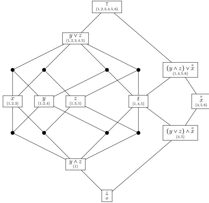
Figure D.27: Resolution of an analogical equation (x : y :: z : t) in a distributive lattice according to Proposition 26. We display an extract of the Boolean lattice of the subsets of \{1, 2, 3, 4, 5, 6\} . Taking x = \{1, 2, 3\} , y = \{1, 2, 4\} and z = \{1, 3, 5\} we have y \wedge z \leq x \leq y \vee z and there exists \hat{x} such that (\hat{x} \vee x \geq y \vee z) and (\hat{x} \wedge x \leq y \wedge z) . Here we choose \hat{x} = \{4, 5, 6\} , but \{1, 4, 5, 6\} and \{1, 4, 5\} are also right. Therefore, t = ((y \vee z) \wedge \hat{x}) \vee (y \wedge z) = ((y \wedge z) \vee \hat{x}) \wedge (y \vee z) = \{1, 4, 5\} is the unique solution to the equation.
