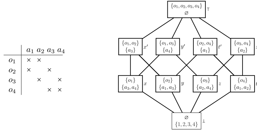
Figure 21: The analogical concept lattice \mathcal{C}_{Analog} and the associated formal context. Concepts x, y, z and t are in complete WAP (through attributes), as well as concepts x', y', z' and t' (through objects).
