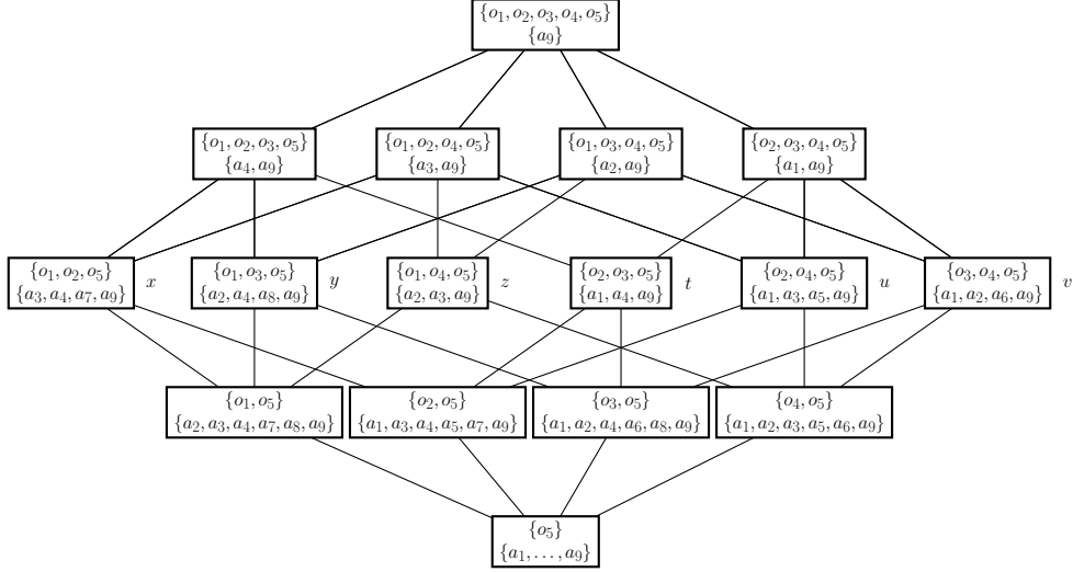
Figure 14: Example of Boolean concept lattice where the FAP x : y :: u : v is not a SAP. The AP \mathbf{o}_x : \mathbf{o}_y :: \mathbf{o}_u : \mathbf{o}_v is true but \mathbf{a}_x : \mathbf{a}_y :: \mathbf{a}_u : \mathbf{a}_v does not hold.
