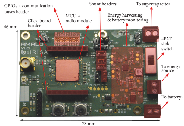
FIGURE 7: Prototype of the energy harvesting LoRa platform.
