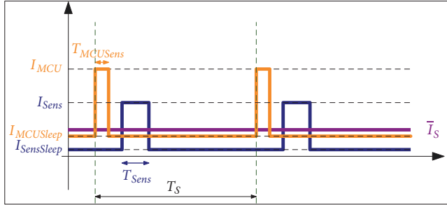
(b) Cycle of a sensing operation: MCU (orange) and sensor (purple) current consumptions
