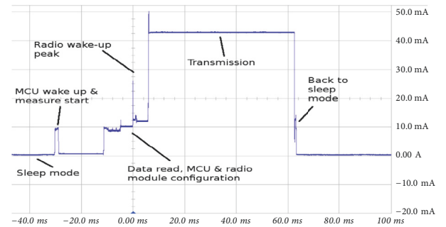
FIGURE 8: Microbenchmark of both MCU and LoRa transmission.
