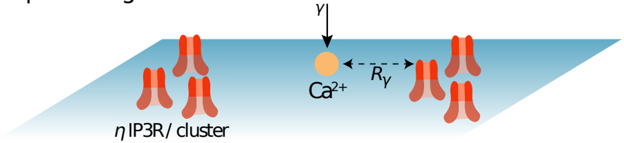
Fig 1. Reaction scheme and IP_3R model The biochemical processes included in the model are illustrated in (A). Cytosolic calcium can exit the cytosol to the extracellular space or the endoplasmic reticulum (ER) at a (total) rate \alpha , lumping together the effects of ER and plasma membrane pumps. Likewise, Ca^{2+} can enter the cytosol from the extracellular space or from the ER via IP_3R -independent flow, with (total) rate \gamma , emulating calcium channels from the plasma membrane. When an IP_3R channel opens, calcium enters the cytosol through the channel at rate \mu . Phospholipase C\delta ( PLC\delta ), once activated by calcium binding, produces IP_3 at rate \delta . Like Ca^{2+} , IP_3 can bind the IP_3R channel and is removed with rate \beta . (B) Our model of the kinetics of the IP_3R channel is an 8-state Markov model adapted from [46, 56]. Each IP_3R channel monomer is associated with 3 binding sites, two calcium binding sites and one IP_3 binding site. Occupancy states are designated by a triplet \{i, j, k\} where i stands for the occupation of the first Ca binding site ( i = 1 if bound, 0 else), j for that of the IP_3 binding site and k for the second Ca site. The first calcium binding site has higher affinity than the second. The open state is state \{110\} , where the first Ca and the IP_3 sites are bound but not the second Ca site. (C) Spatial parameters for the particle-based model. The N_{IP_3R} IP_3R molecules are positioned within uniformly distributed clusters, with \eta IP_3R in each cluster. Hence \eta = 1 corresponds to uniformly distributed IP_3R (no clustering), while the degree of clustering increases with \eta (for constant total IP_3R number). To account for potential co-localization between IP_3R -dependent and IP_3R -independent calcium sources, the influx of IP_3R -independent calcium (at rate \gamma ) occurs within distance R_\gamma of an IP_3R . Thus, low values of R_\gamma emulate co-localization between IP_3R -dependent and IP_3R -independent Ca^{2+} influx sources.
