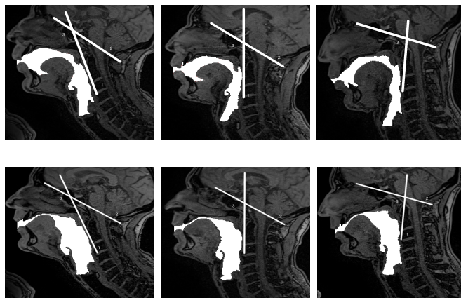
Figure 2. 2D segmentation of /o/ (top row) and /i/ (bottom row) vowels at up, normal and down position from left to right. Lines 1 and 2 are used to define the angle \theta of the head position
