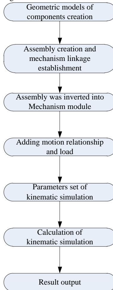
Fig. 2. Process of kinematic simulation in Creo Parametric
