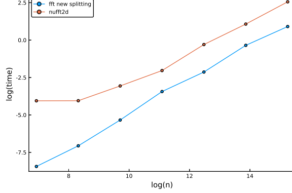
FIGURE 7. Time execution as a function of the total number of points (log – log scale). Blue: new method (new splitting and one-dimensional fast Fourier transform). Red: exact computation of the feet of the characteristics and two-dimensional non uniform fast Fourier transform.
