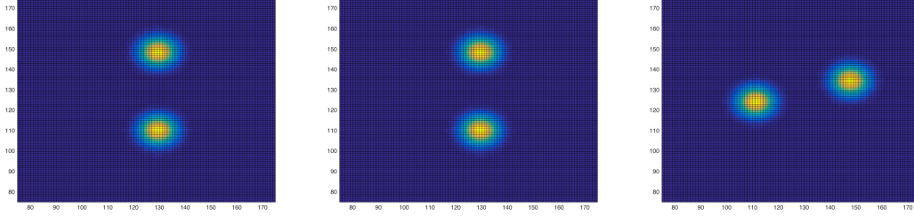
FIGURE 3. Solution u(T, x) of (2.28). Left: Exact solution u(T, x) . Middle: Numerical solution obtained by the new splitting. Right: Numerical solution obtained by the Strang splitting.
