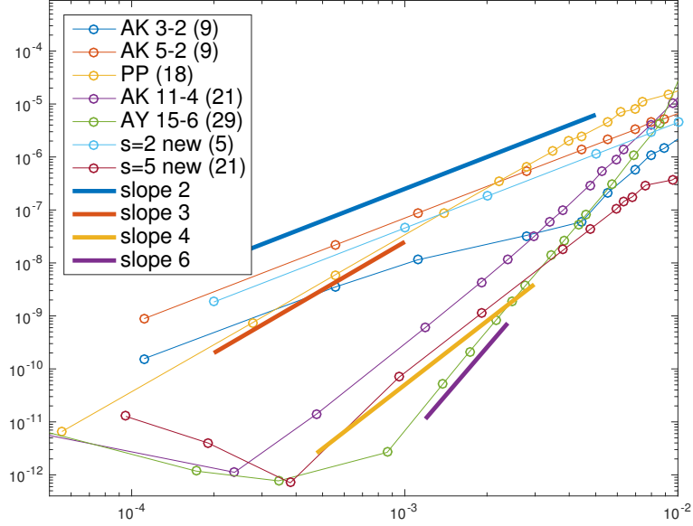
FIGURE 10. Efficiency diagrams obtained by different methods from [2] and \psi_{\delta_t}^{[2]} , \psi_{\delta_t}^{[5]} for the Vlasov–Maxwell system. The order lines ‘slope 2’ and ‘slope 4’ are the same as in Figure 8. The number of maps for each method is indicated into parenthesis.
