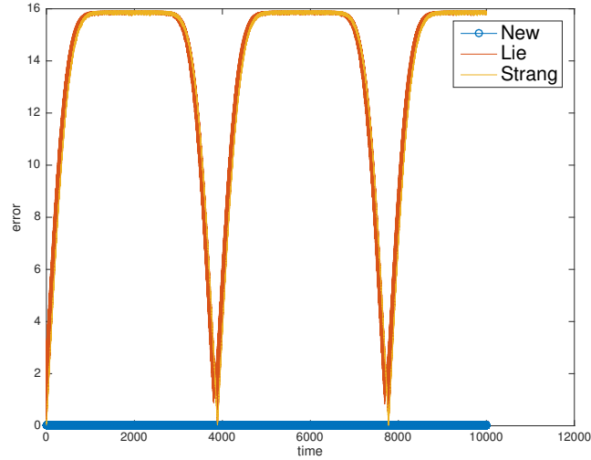
FIGURE 4. Time history of the relative errors between the exact solution of (2.28) and the numerical solution obtained by the new splitting ('New'), the Lie splitting ('Lie') and the Strang splitting ('Strang').
