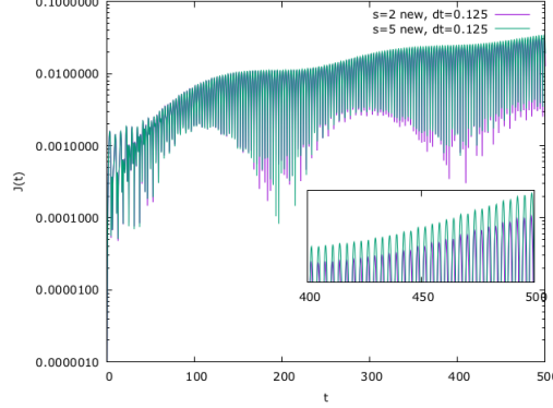
FIGURE 12. Time history of the first mode of E_1 (semi-log scale): \psi_{\delta_t}^{[2]} and \psi_{\delta_t}^{[5]} with \delta_t = 0.125 .
