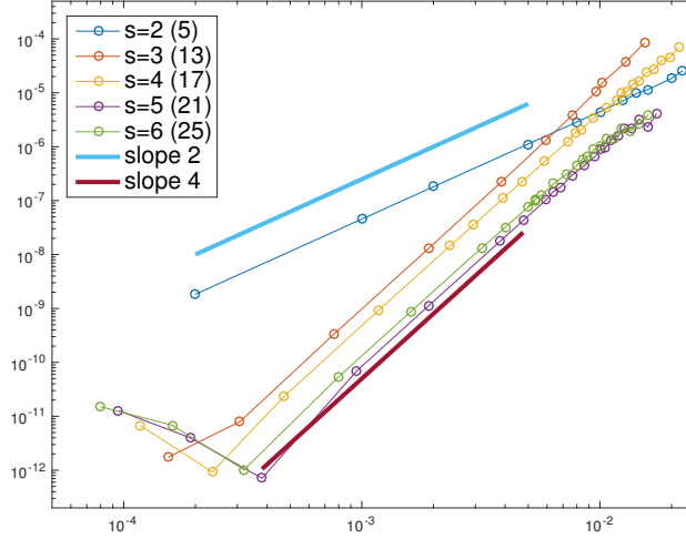
FIGURE 8. Efficiency diagrams obtained by different composition methods \psi_{\delta_t}^{[s]} , s = 2, 3, 4, 5, 6 for the Vlasov–Maxwell system. The number of maps for each method is indicated into parenthesis.
