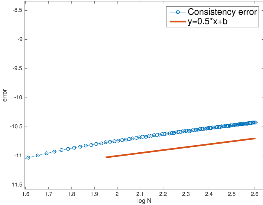
FIGURE 2. Zoom of Figure 1.
