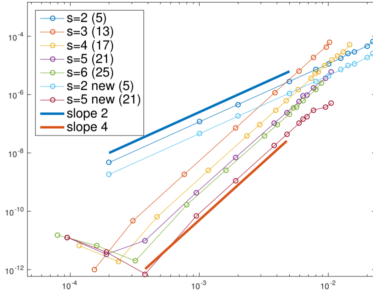
FIGURE 9. Efficiency diagrams obtained by different composition methods \tilde{\psi}_{\delta_t}^{[s]} , s = 2, 3, 4, 5, 6 and \psi_{\delta_t}^{[2]} , \psi_{\delta_t}^{[5]} for the Vlasov–Maxwell system. The order lines ‘slope 2’ and ‘slope 4’ are the same as in Figure 8. The number of maps for each method is indicated into parenthesis.
