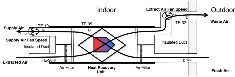
Fig. 1: Schematic diagram of air handling unit
