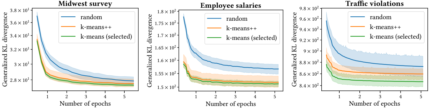
Fig. 10: Convergence for different initializations for the Gamma-Poisson model. In all experiments, the k-means strategy is used.
