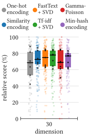
Fig. 7: All encoders perform well for low-cardinality datasets. Classifier: XGBoost.
