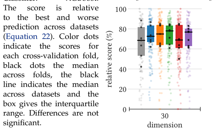
Fig. 7: All encoders perform well for low-cardinality datasets. Classifier: XGBoost. The score is relative to the best and worse prediction across datasets (Equation 22). Color dots indicate the scores for each cross-validation fold, black dots the median across folds, the black line indicates the median across datasets and the box gives the interquartile range. Differences are not significant.
