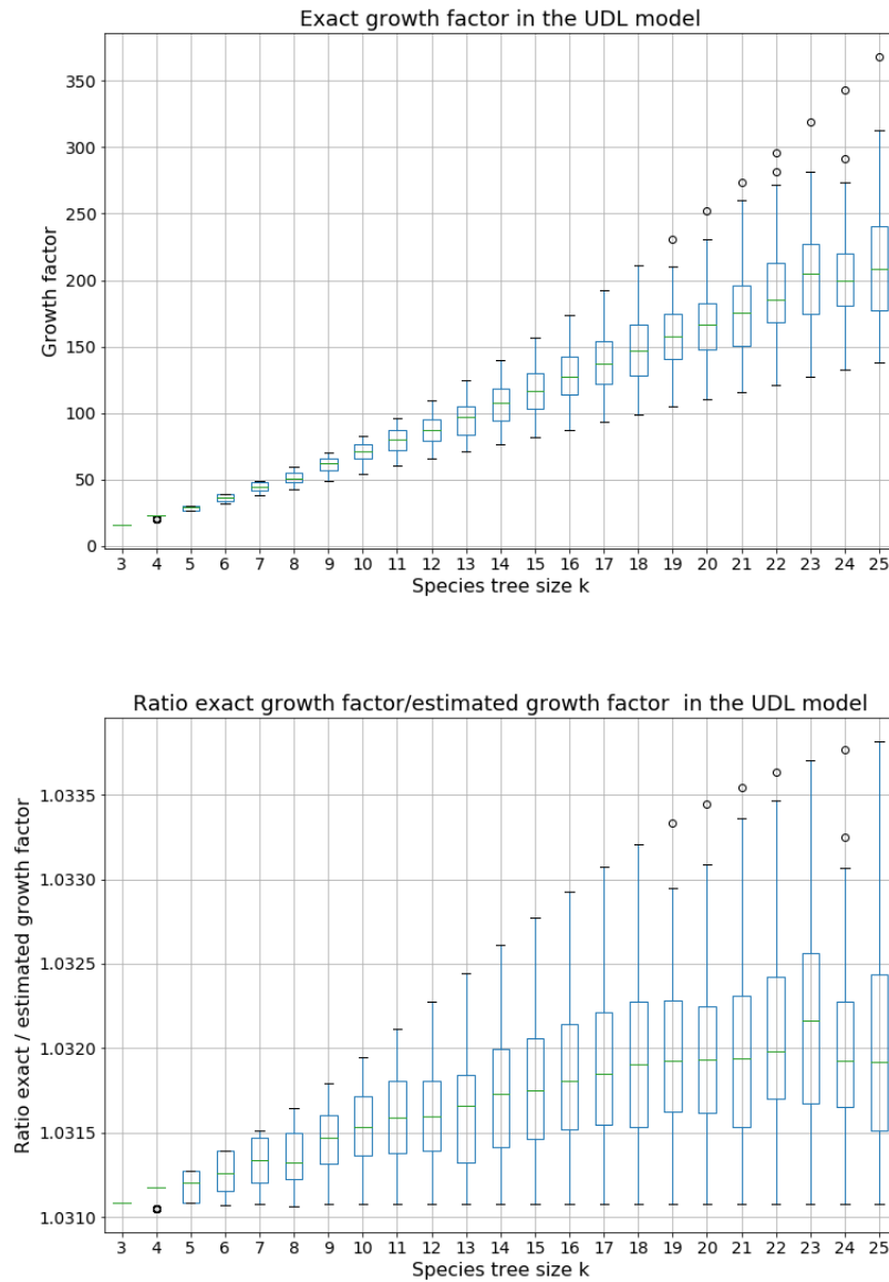
Fig. 5: Box-plot of the distribution of the growth factor for each 100 random species tree per size k in the uDL -model. (Top) Exact growth factor; (Bottom) Box-plot of the distribution, for each species tree, of the ratio between the exact growth factor and the estimated growth factor.
