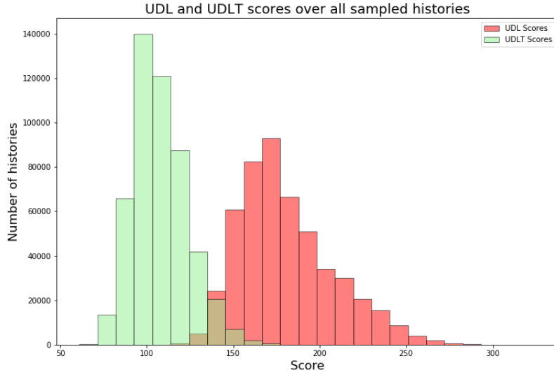
Fig. 9: Distribution of the score (number of duplications plus losses plus HGT) over 50 random species trees of size 16 and 10,000 random histories of size 30 per tree in the \mathbf{uDL} - and \mathbf{uDLT} -models.
