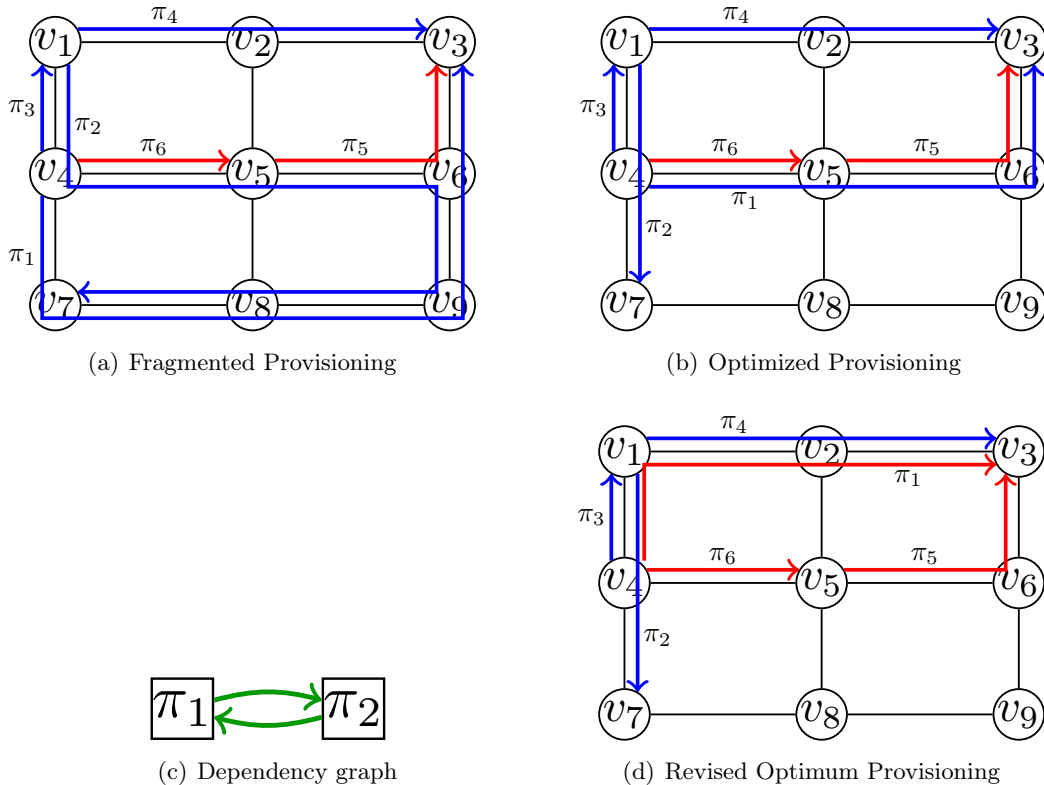
Figure 3: Preprocessing Operation
