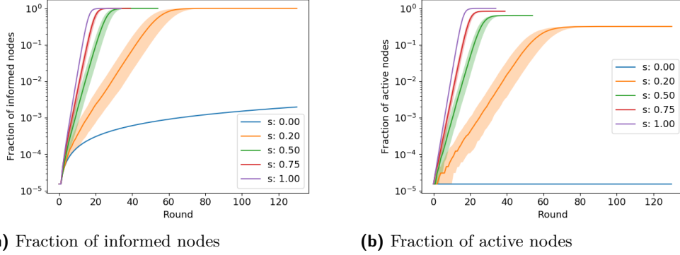
■ Figure 2 Effect of parameter s of Algorithm 1 on the spreading time for a network of n = 2^{16} nodes. The curves represent median values and the shaded area represents the 10 and 90 percent confidence intervals over 100 runs. Each curve stops when all nodes are informed (and so the protocol terminates), except for s = 0 since the protocol is very slow in this case.
